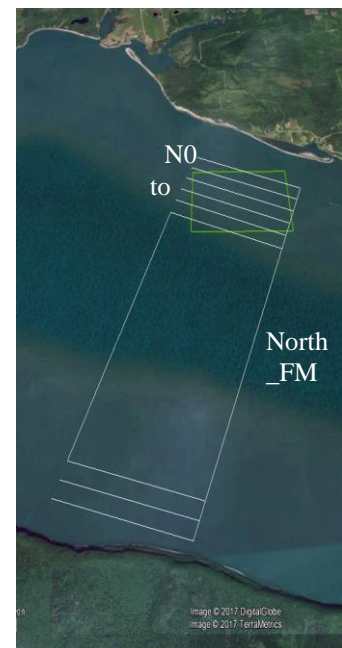
Figure 4: Contemporary survey grid. The green square represents the CLA. White lines show one complete grid, with transects at the CLA (N0-N5) and reference (S1-S3) sites connected by cross-channel transects (South_CW and North_FM).
