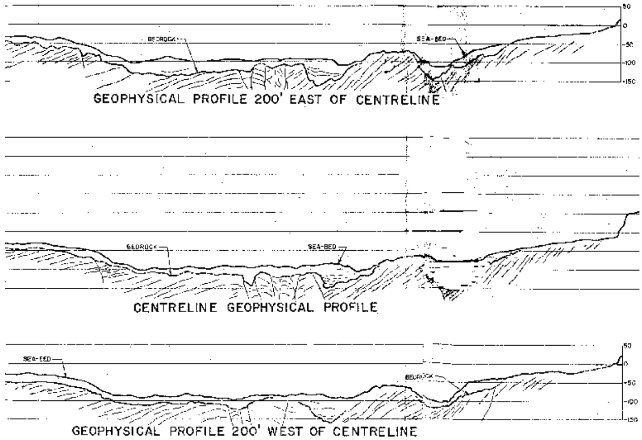
Figure 5.4-5. Three channel cross-sections at the entrance to Cobequid Bay, suggesting that seafloor geology is locally quite variable.
