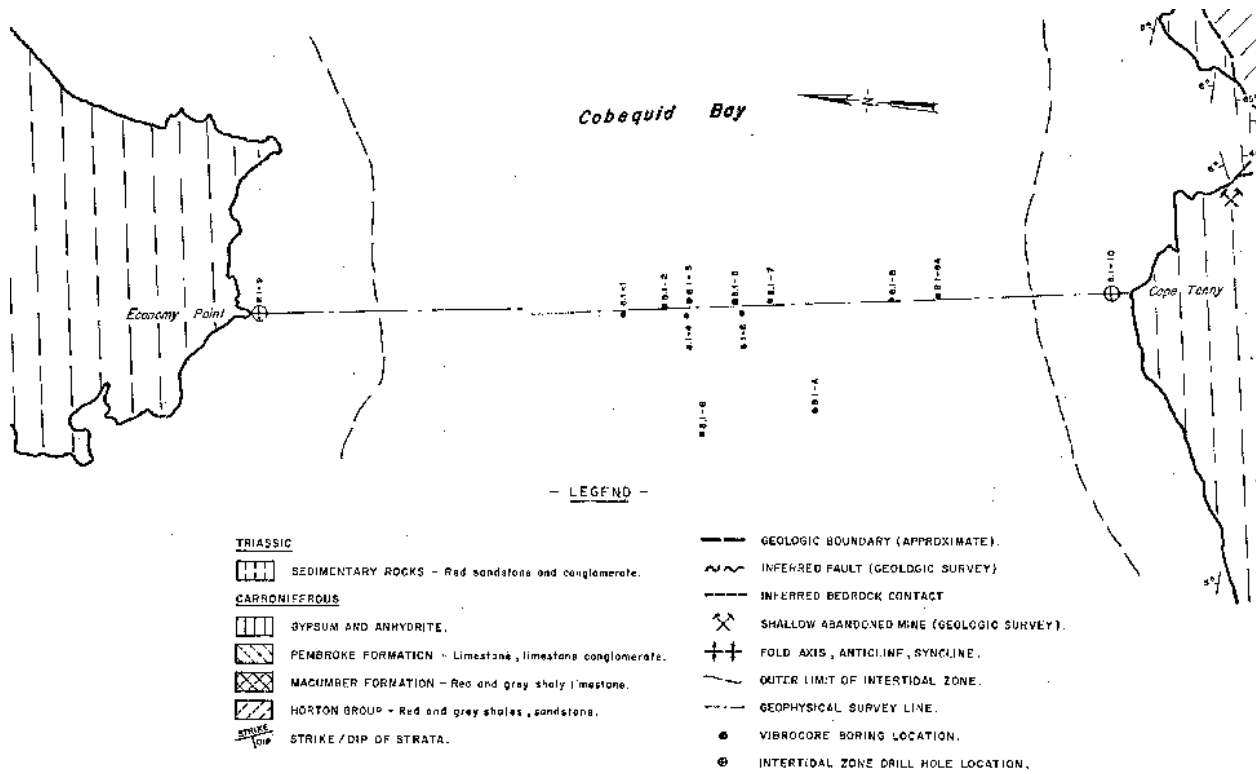
Figure 5.4-4. Geophysical survey at the entrance to Cobequid Bay, between Economy Point and Cape Tenny.
