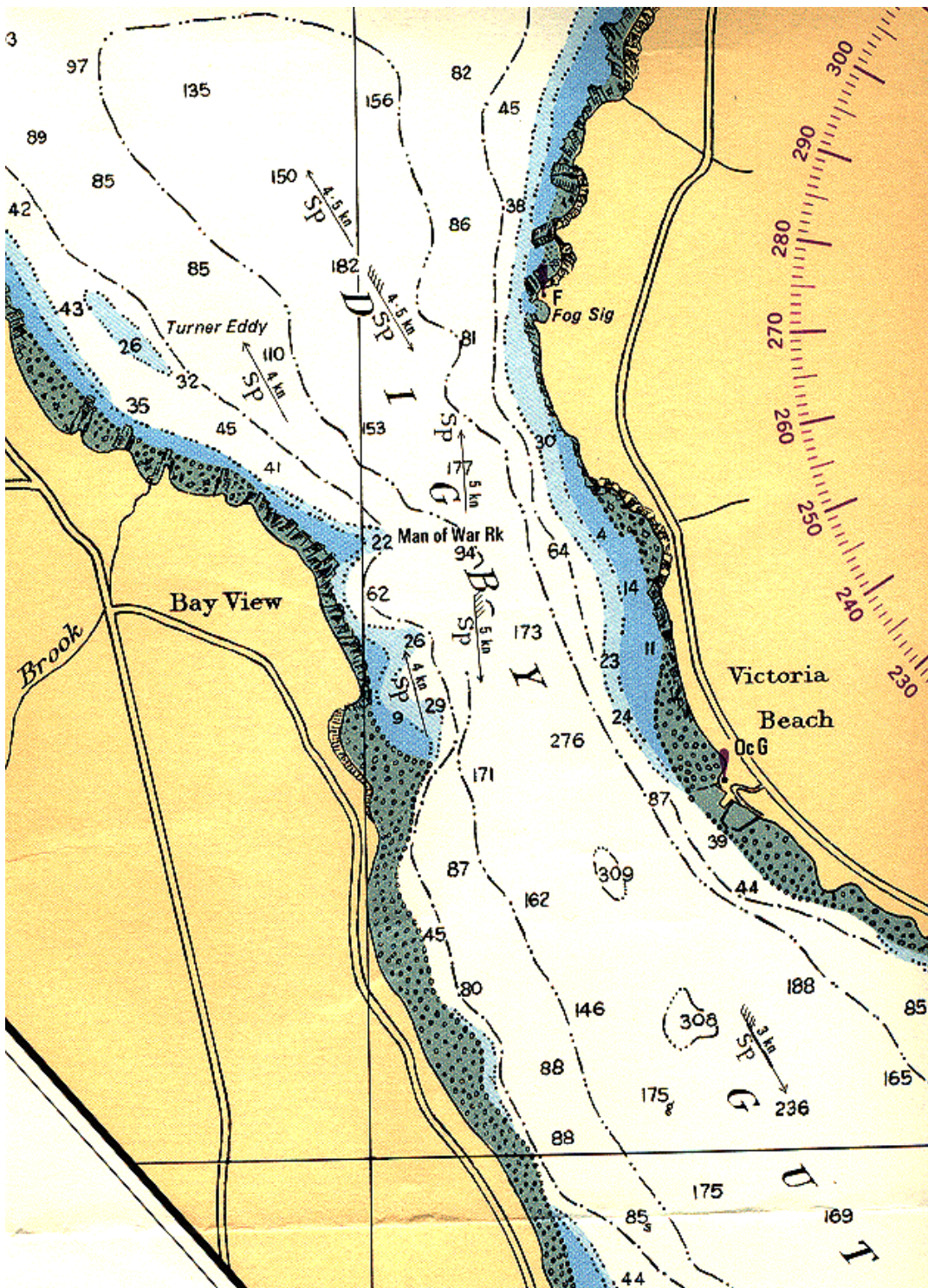
Figure 5.5-5. Scanned section of CHS chart #4396 for Digby Gut. Depths are in feet (1 ft = 0.3 m).
