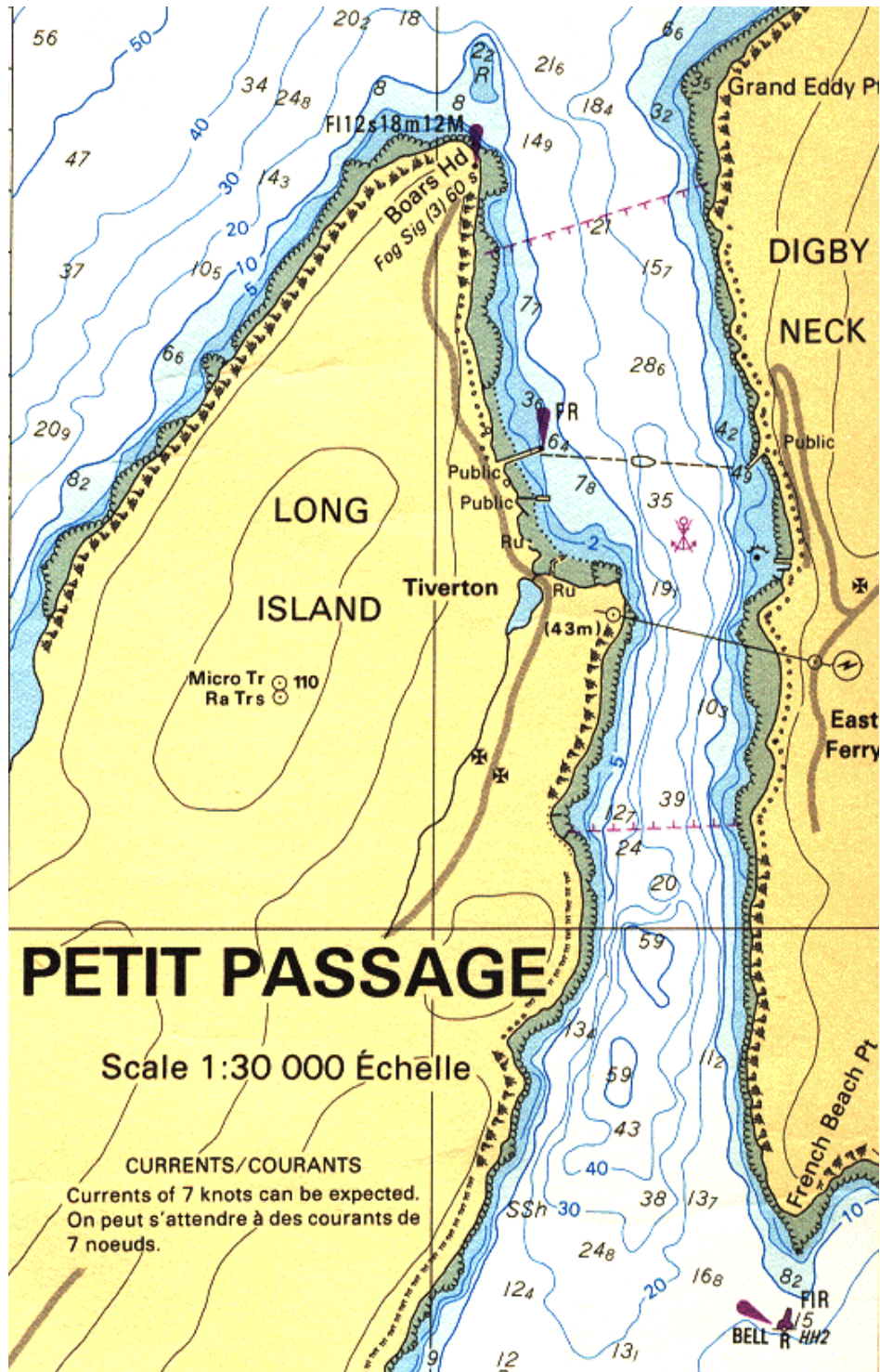
Figure 5.6-3. Scanned section of CHS chart #4118 for Petit Passage. Depths are in meters (1 m = 3.3 ft).
