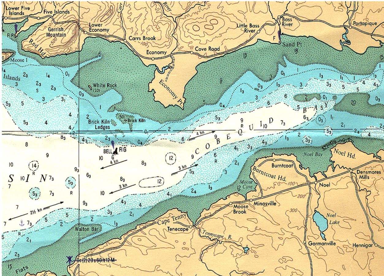
Figure 5.4-3. Scanned section of CHS chart #4010 for Cobequid Bay. Depths are in fathoms, with additional feet as subscript (1 fathom = 6 ft = 1.8 m).
