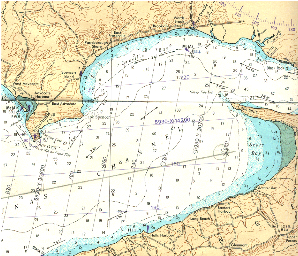
Figure 5.2-3. Scanned section of CHS chart #4010 for Minas Channel. Depths are in fathoms, with additional feet as subscript (1 fathom = 6 ft = 1.8 m).
