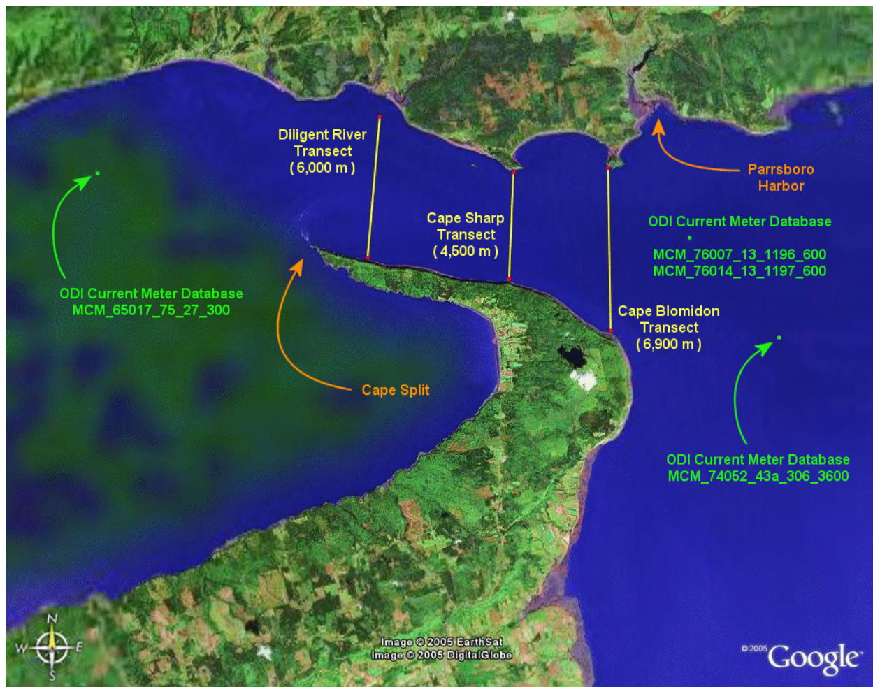
Figure 5.3-2. Aerial photograph from an altitude of approximately 30 km, showing the numerically modeled transects in Minas Passage (Reference 6).
