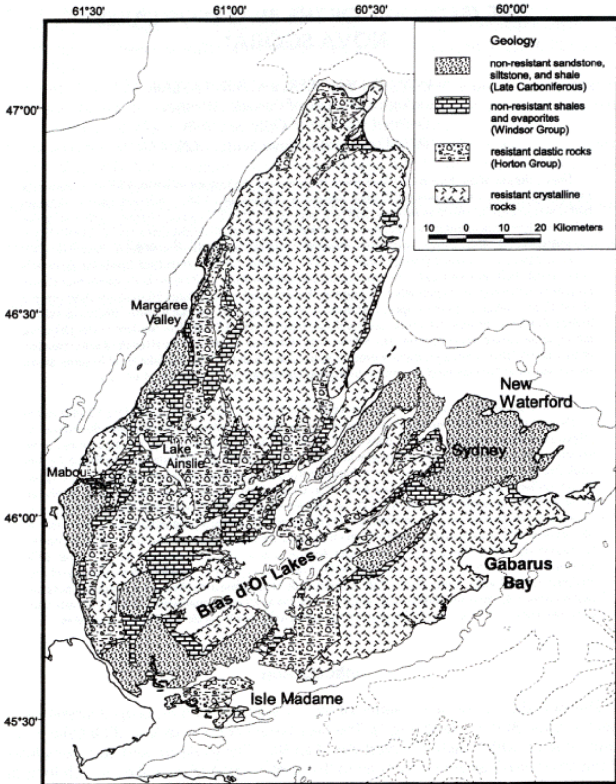
Figure 5.8-3. Regional bedrock geology adjacent to Great Bras d'Or Channel.
