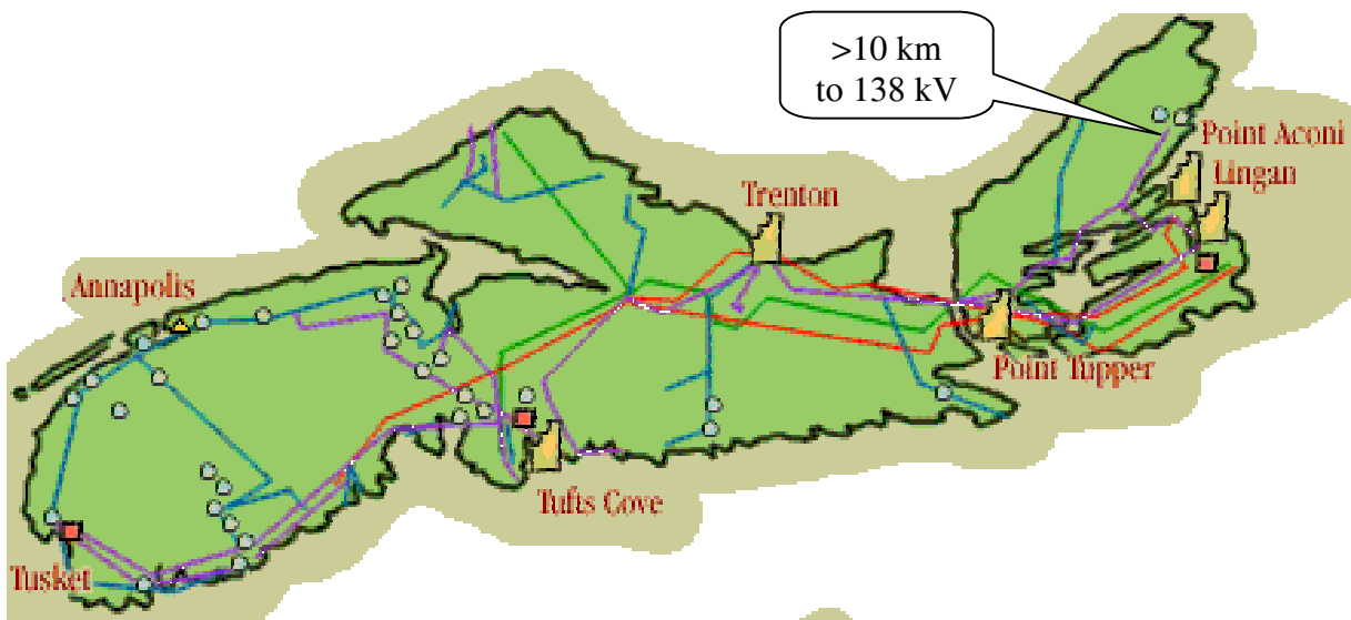
Figure 5.8-5 Distance from Site to transmission connection
