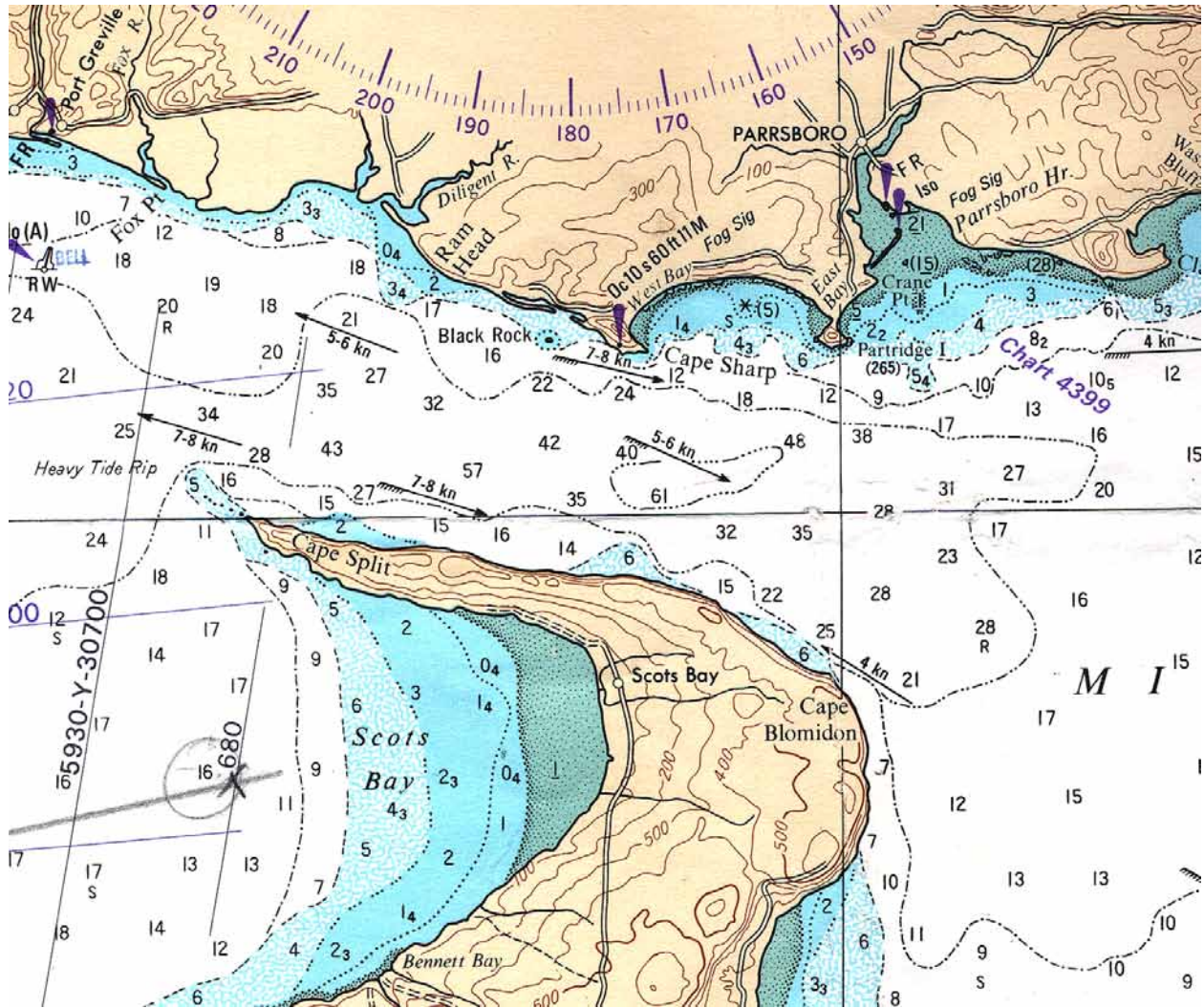
Figure 5.3-3. Scanned section of CHS chart #4010 for Minas Passage. Depths are in fathoms, with additional feet as subscript (1 fathom = 6 ft = 1.8 m).
