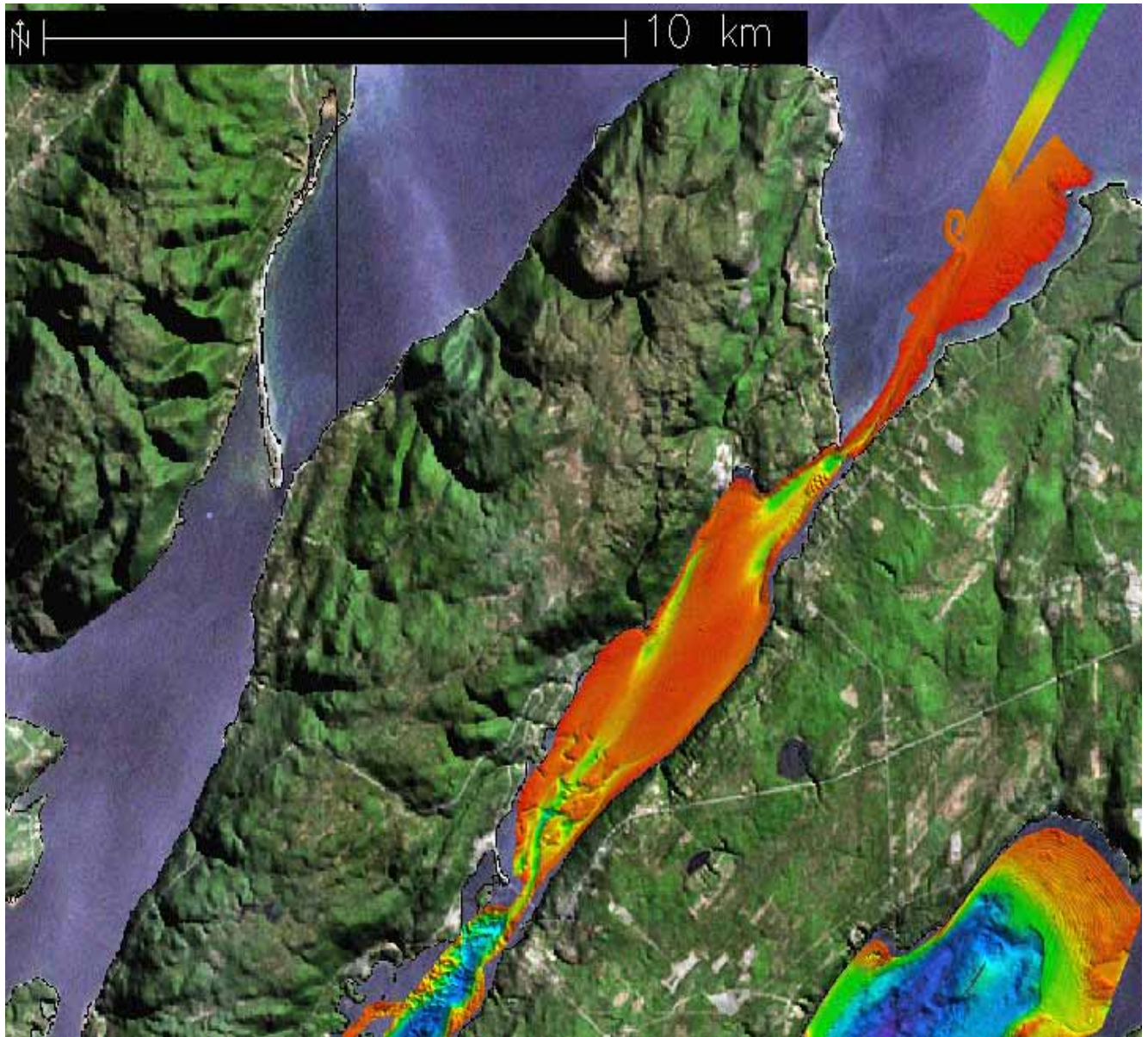
Figure 5.8-4. Multibeam imagery of Great Bras d'Or Channel
