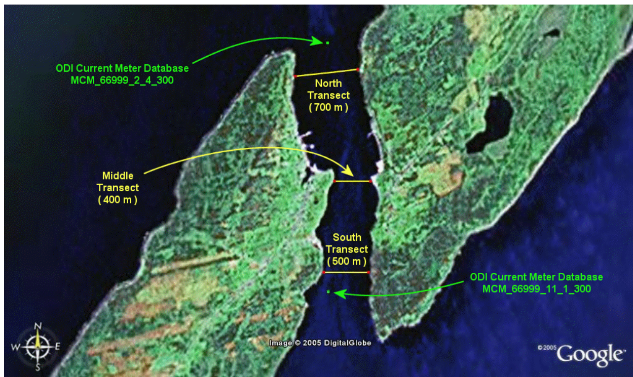
Figure 5.6-2. Aerial photograph from an altitude of approximately 6 km, showing the numerically modeled transects in Petit Passage (Reference 6).
