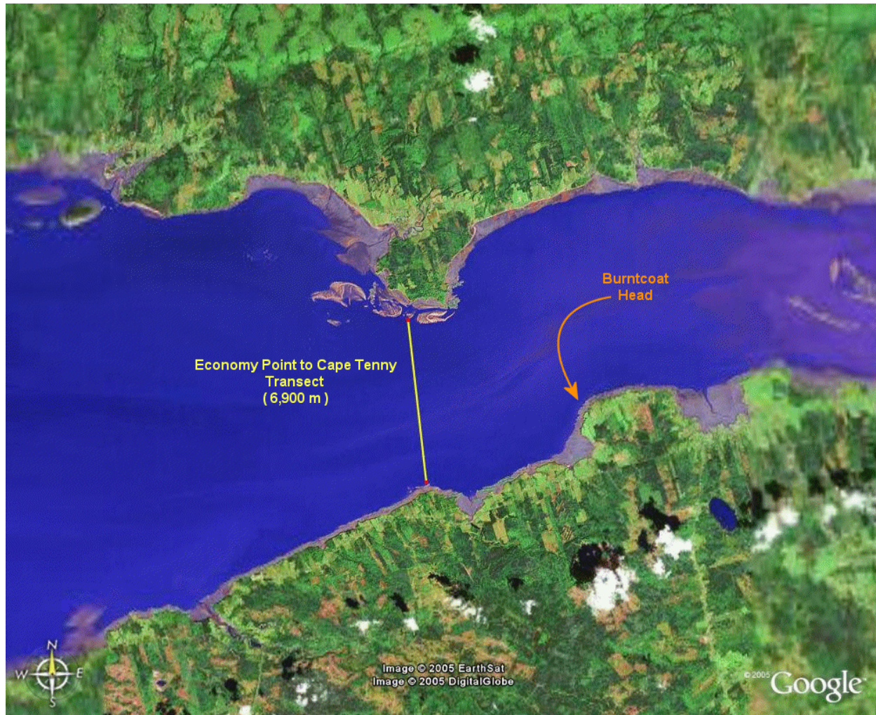
Figure 5.4-2. Aerial photograph from an altitude of approximately 20 miles, showing the numerically modeled transect in Cobequid Bay (Reference 6).
