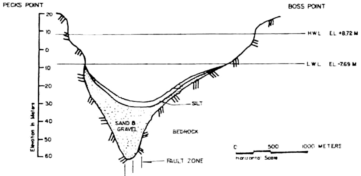
Figure 5.1-4. Sediment thickness in Cumberland Basin transect between Pecks Point, New Brunswick and Boss Point, Nova Scotia. The sediment overburden is 10 m or less in the eastern half of the transect, and up to 40 m thick in the buried river valley of the western half.
