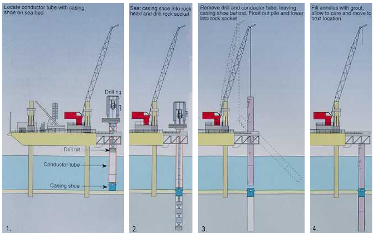
Figure 4.1-1. Monopile foundation installation sequence.
