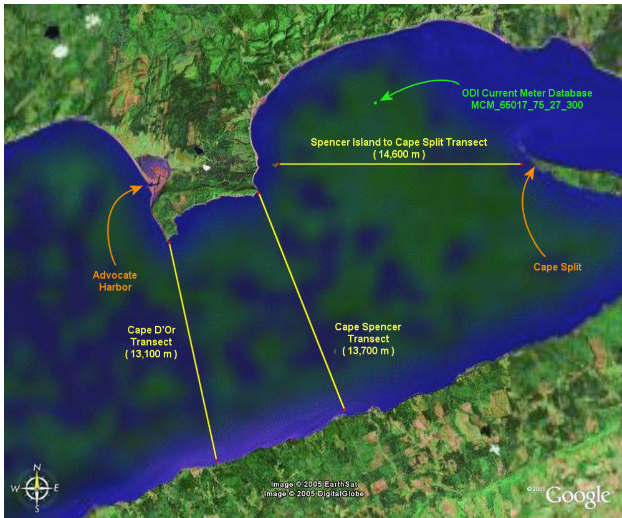
Figure 5.2-2. Aerial photograph from an altitude of approximately 30 km, showing the numerically modeled transects in Minas Channel (Reference 6).
