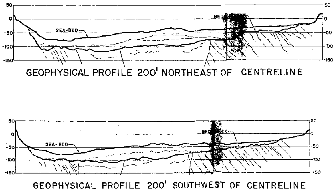
Figure 5.1-6. Additional channel cross-sections at Cumberland Basin entrance, suggesting uniformity of seafloor geology over a broad area.
