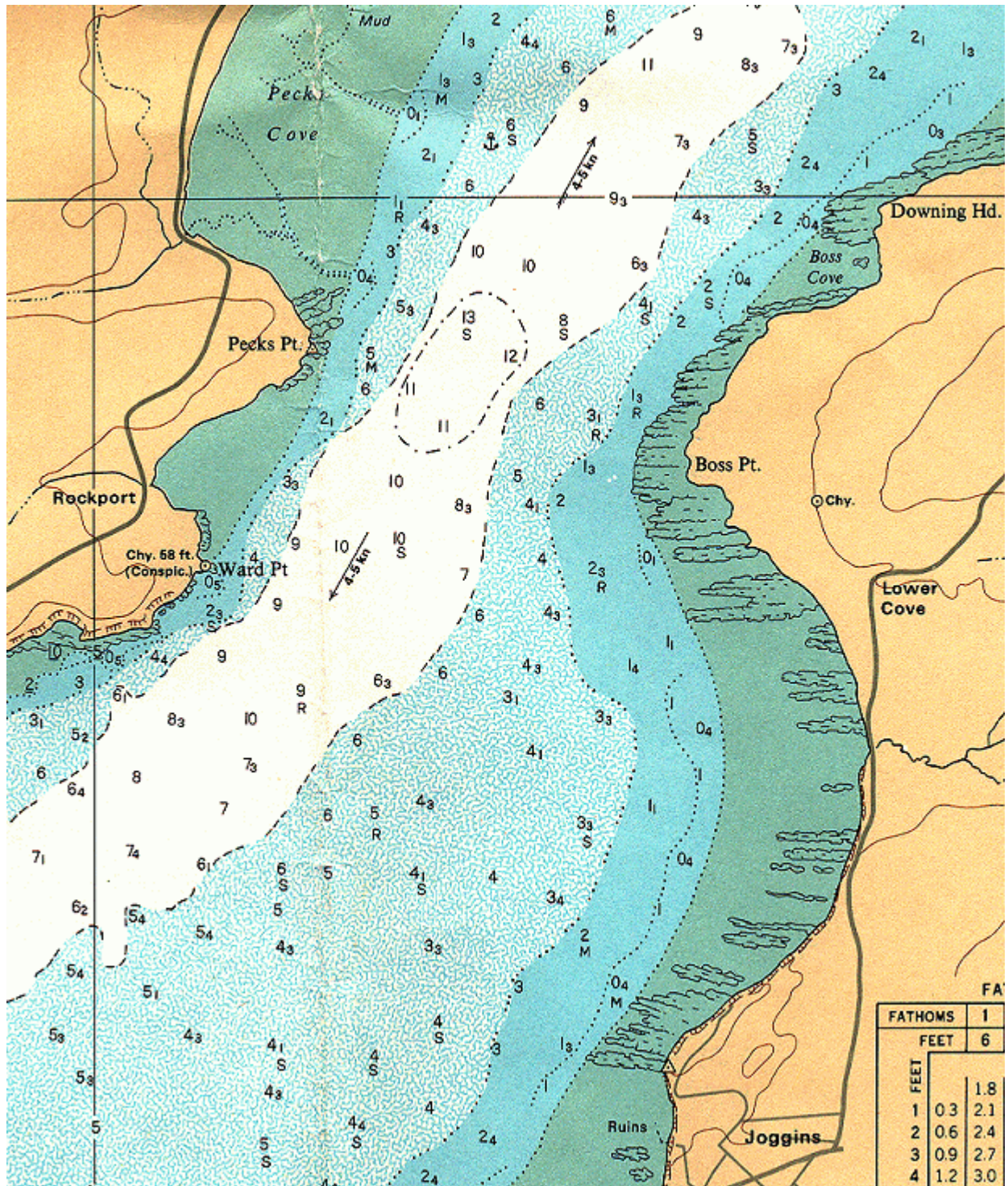
Figure 5.1-3. Scanned section of CHS chart #4130 for Cumberland Basin. Depths are in fathoms, with additional feet as subscript (1 fathom = 6 ft = 1.8 m).
